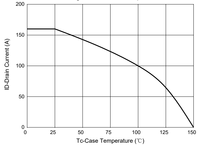
Fig. 10 - Current dissipation
