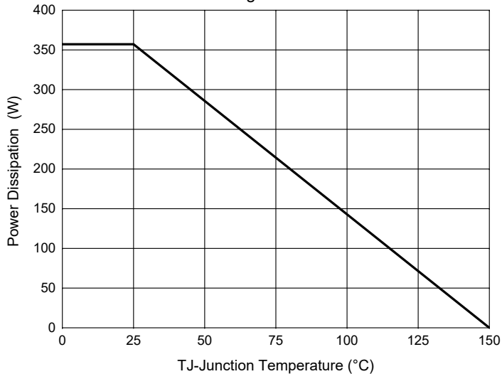
Fig.11-PD-TJ
