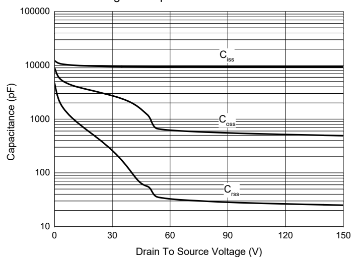
Fig. 5 - Capacitance Characteristics
