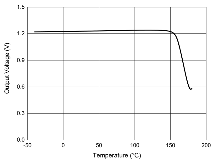
Fig. 4 - MCT1117C-ADJ Thermal Performance with OTP
