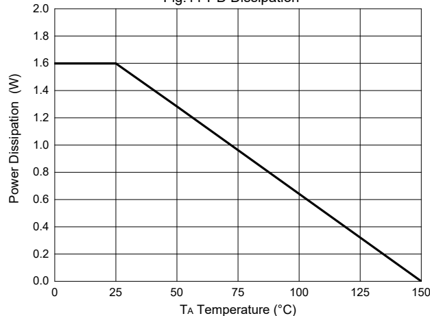
Fig.11-PD Dissipation
