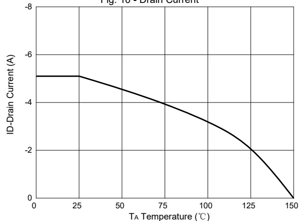
Fig. 10 - Drain Current
