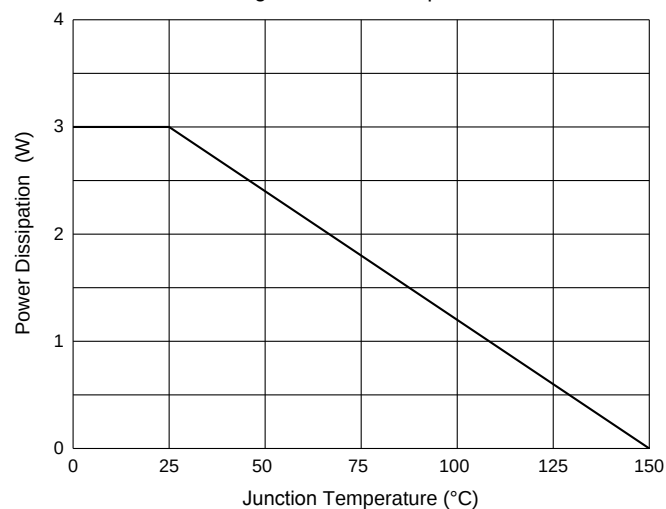
Fig. 4 - Power Dissipation
