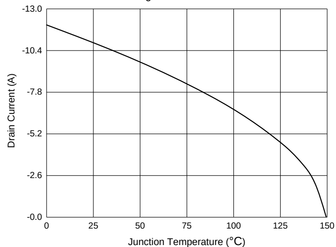
Fig. 3 - Drain Current
