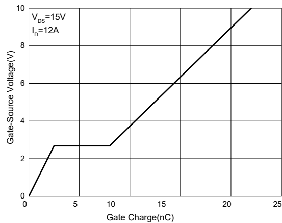
Fig.6 - Gate Charge
