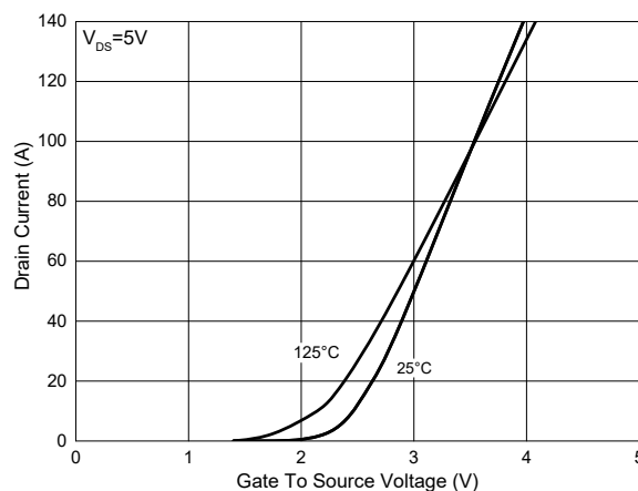
Fig.2 - Transfer Characteristic
