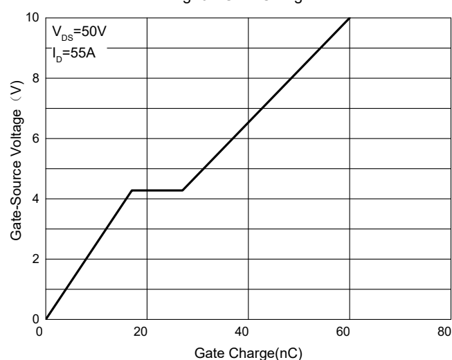
Fig. 6 - Gate Charge
