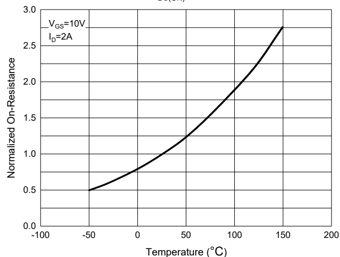
Fig. 5 - R_{DS(ON)} - \text{Temperature}
