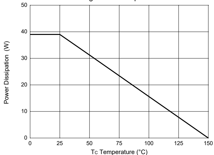
Fig.11-PD Dissipation
