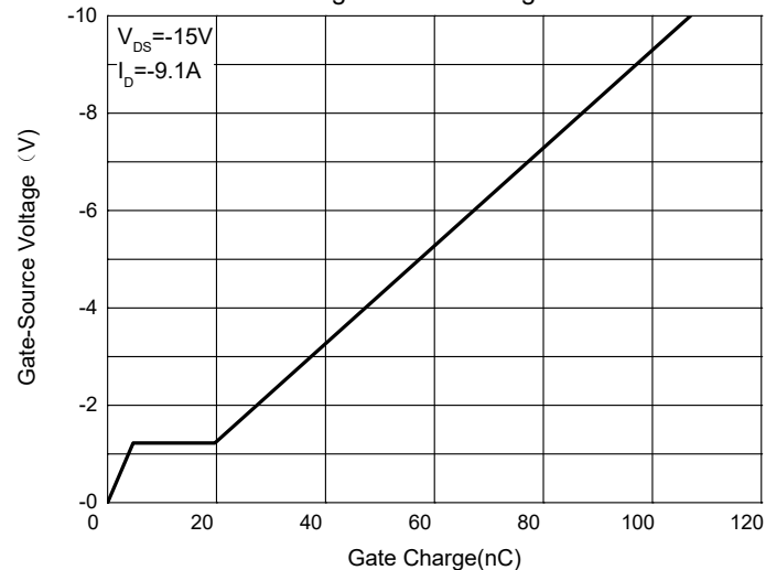
Fig. 6 - Gate Charge
