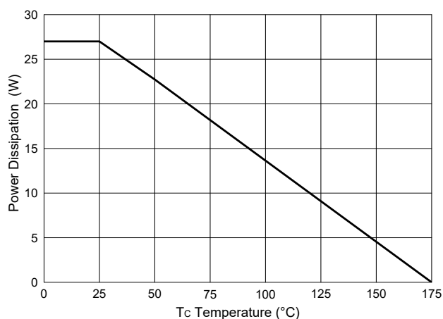
Fig.11-PD Dissipation
