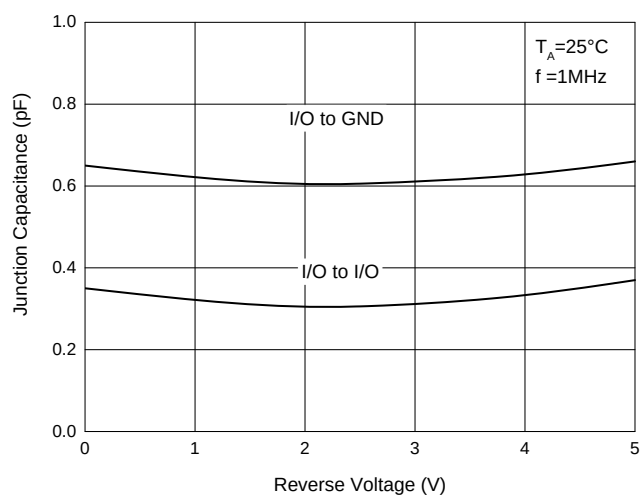
Fig. 4 - Capacitance Characteristics
