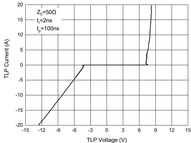
Fig. 6 - TLP Measurement
