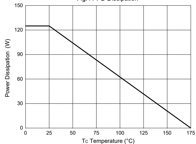
Fig.11-PD Dissipation
