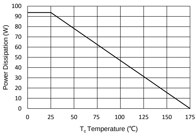
Fig.11 - PD Dissipation
