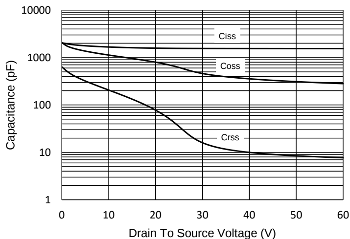
Fig.5 - Capacitance Characteristics
