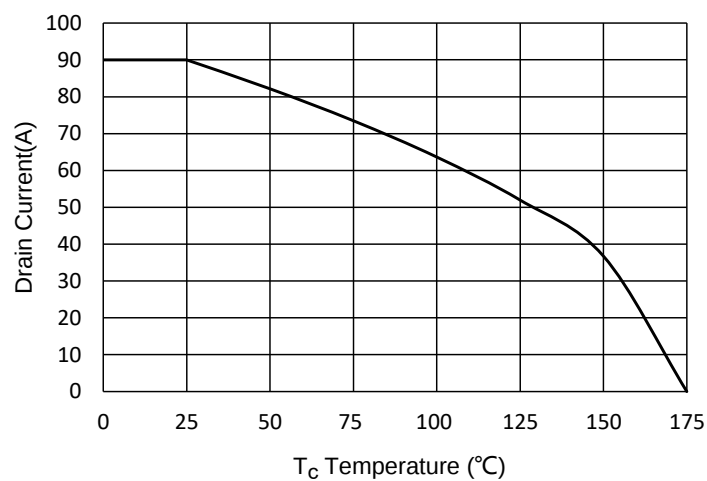
Fig.10 - Drain Current
