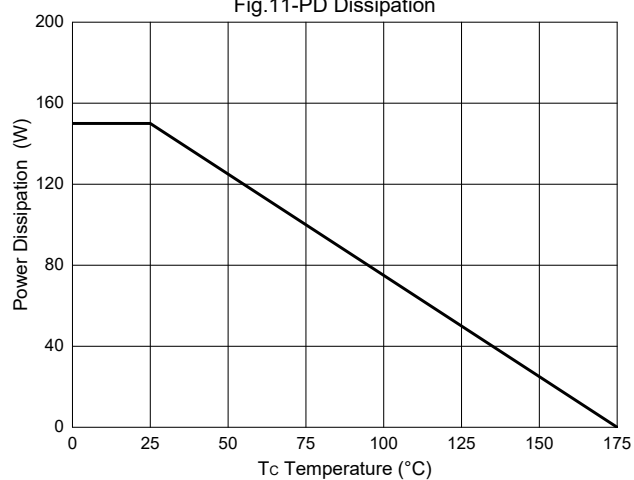
Fig.11-PD Dissipation
