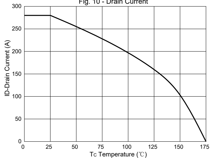
Fig. 10 - Drain Current
