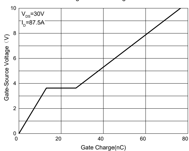
Fig. 6 - Gate Charge
