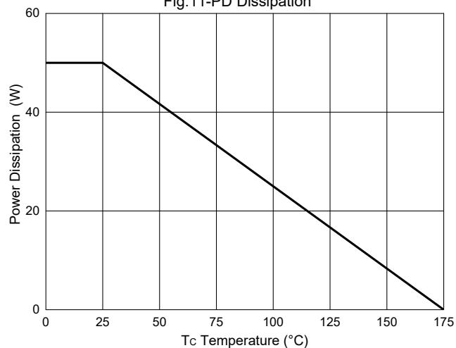
Fig.11-PD Dissipation
