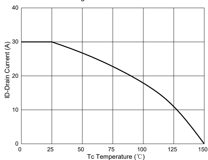
Fig. 10 - Drain Current
