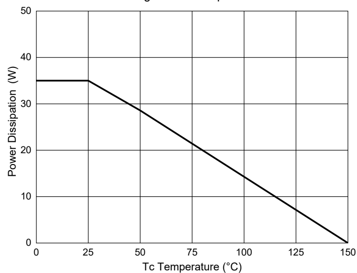
Fig.11-PD Dissipation
