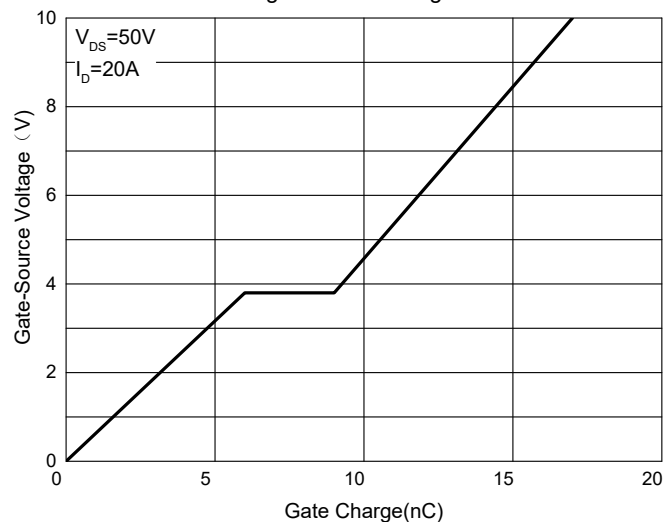
Fig. 6 - Gate Charge
