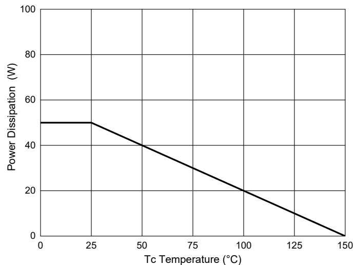
Fig.11-PD Dissipation
