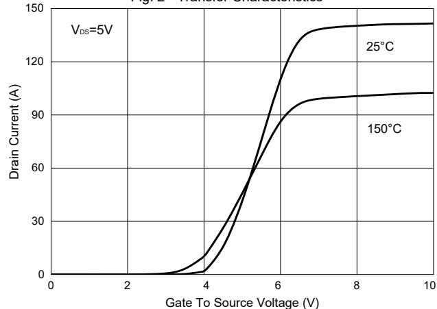
Fig. 2 - Transfer Characteristics
