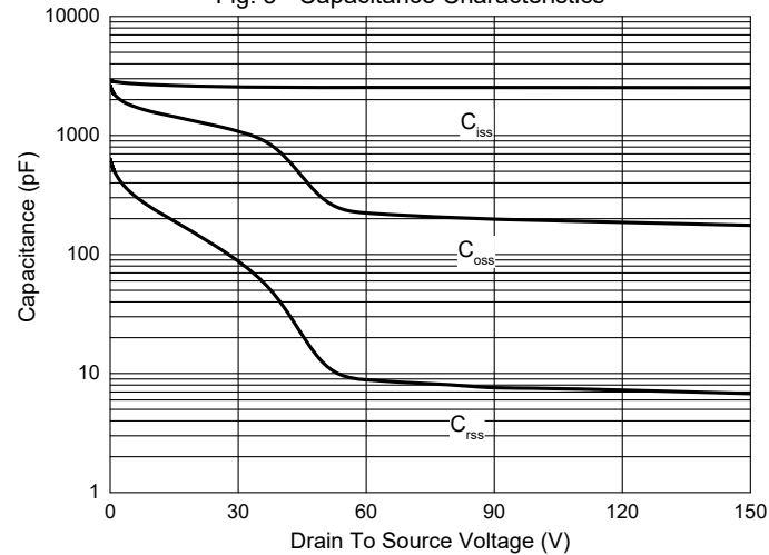
Fig. 5 - Capacitance Characteristics
