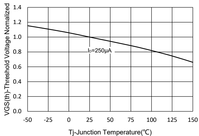
Fig.7-Normalized Threshold Voltage
