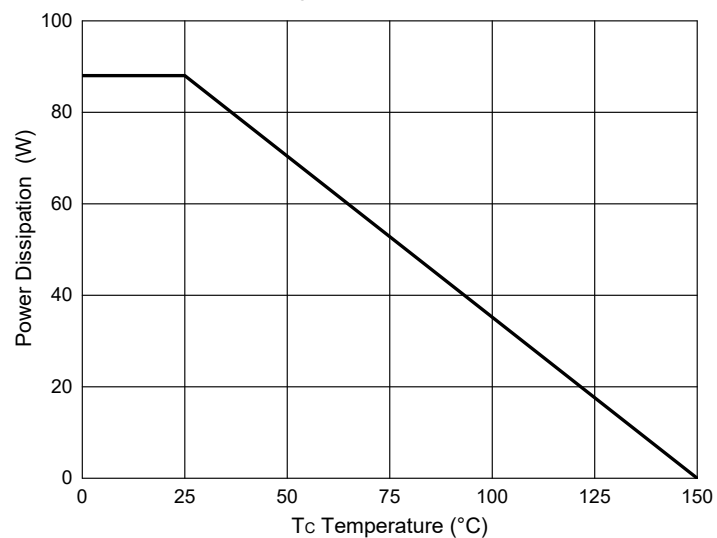
Fig.11-PD Dissipation
