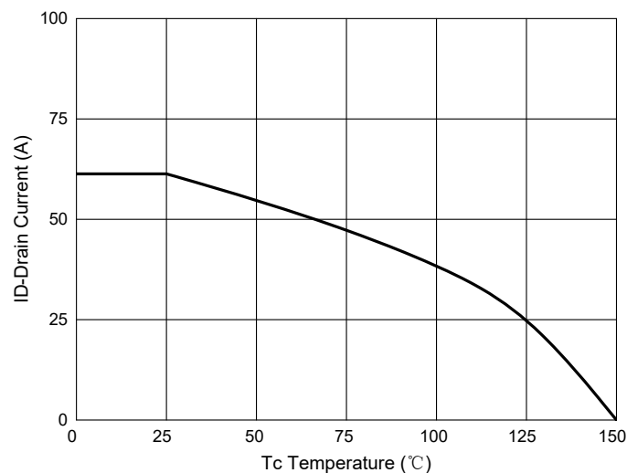
Fig. 10 - Current dissipation
