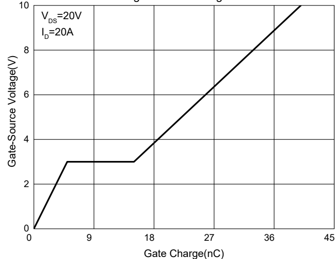
Fig. 6 - Gate Charge
