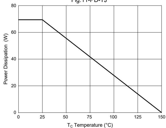
Fig.11-PD-TJ
