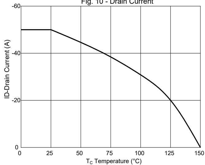
Fig. 10 - Drain Current
