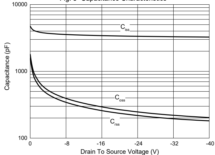
Fig. 5- Capacitance Characteristics
