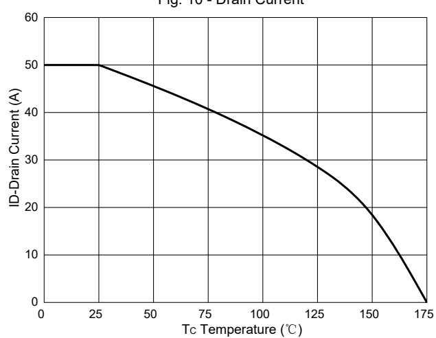
Fig. 10 - Drain Current
