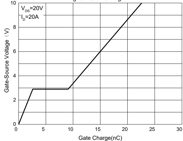
Fig. 6 - Gate Charge
