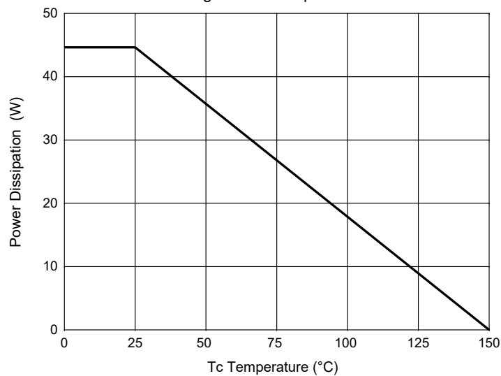
Fig.11-PD-Dissipation
