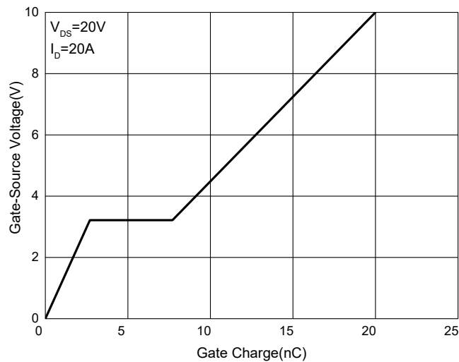
Fig. 6 - Gate Charge
