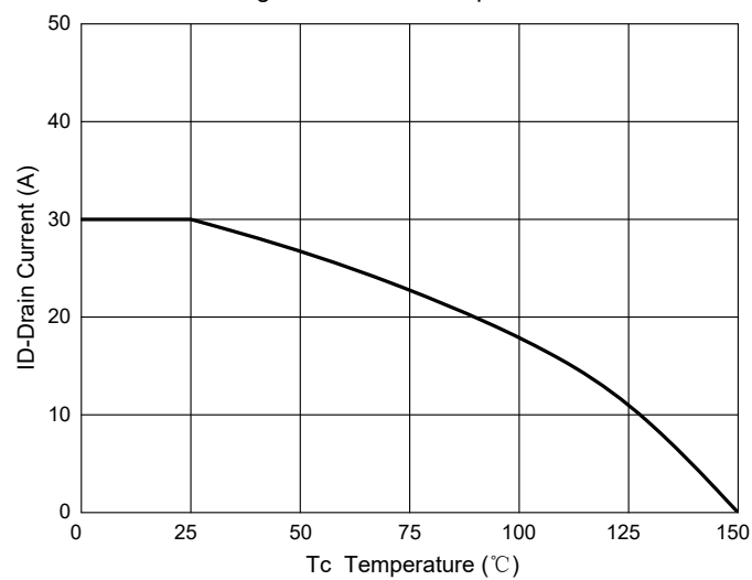
Fig. 10 - Current dissipation
