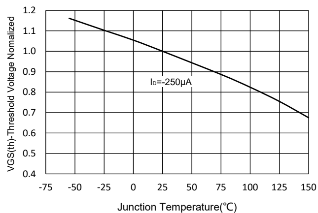
Fig.7 Threshold Voltage
