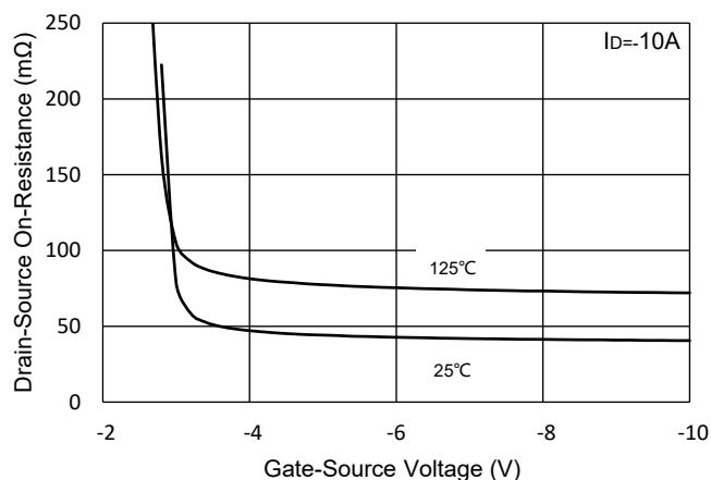
Fig.3 Rdson-Vgs
