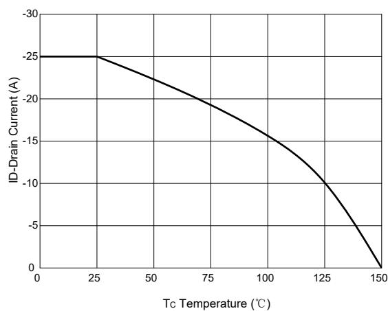
Fig. 10 - Drain Current
