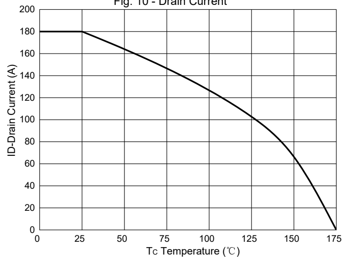
Fig. 10 - Drain Current
