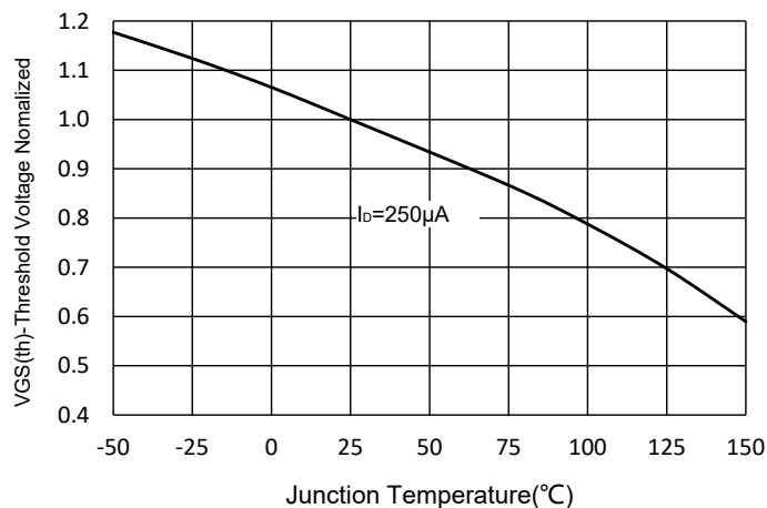
Fig.7 Threshold Voltage
