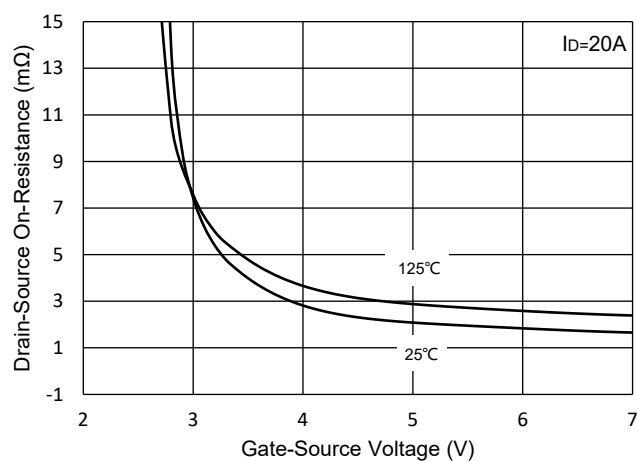
Fig.3 Rdson-Vgs
