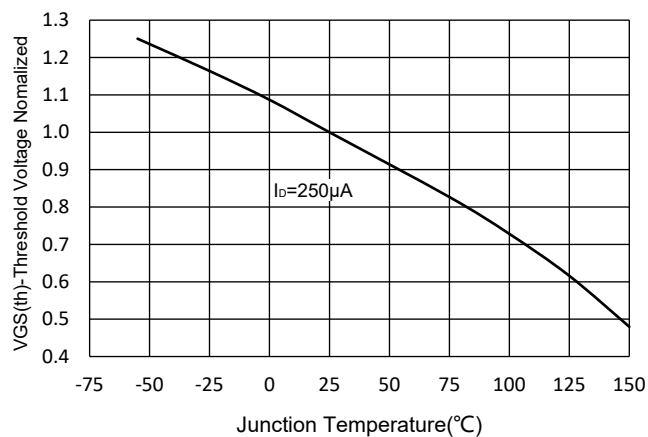
Fig.7 Threshold Voltage
