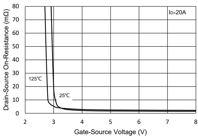
Fig.3 Rdson-Vgs
