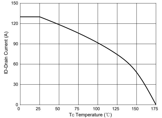
Fig. 10 - Drain Current
