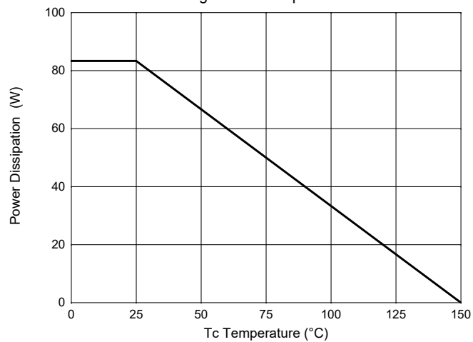
Fig.11-PD Dissipation
