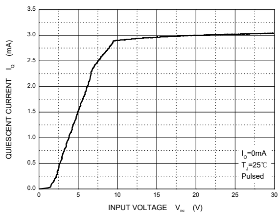
Fig.3 Quiescent Current vs Input Voltage
