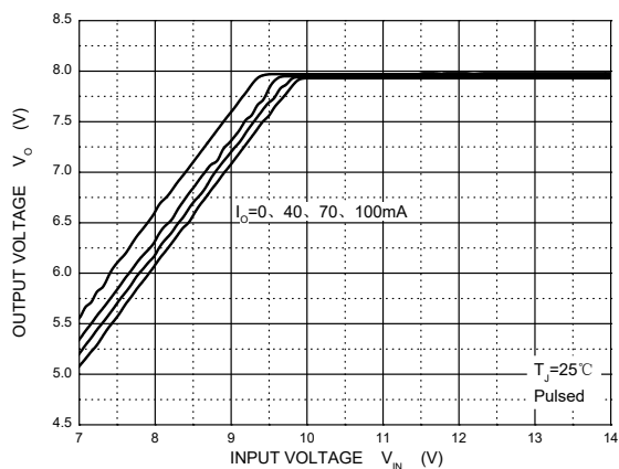
Fig.2 Dropout Characteristics
