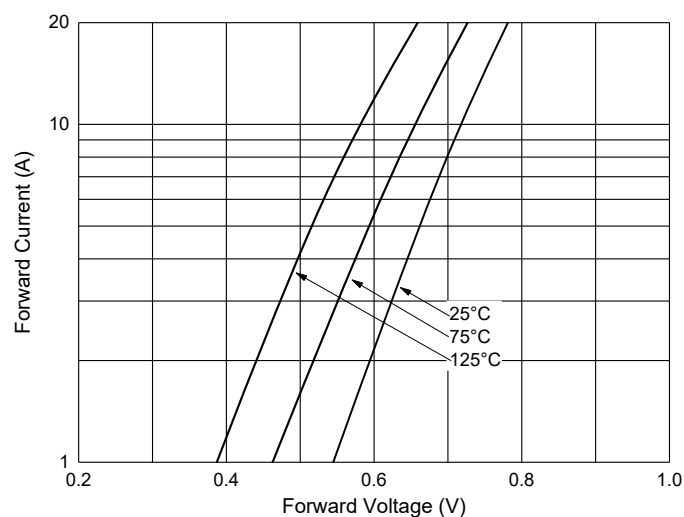
Fig. 3 - Forward Characteristics
