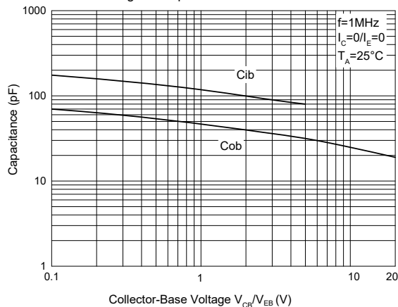
Fig. 5 - Capacitance Characteristics
