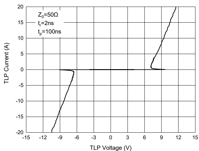
Fig. 3 - TLP Measurement
