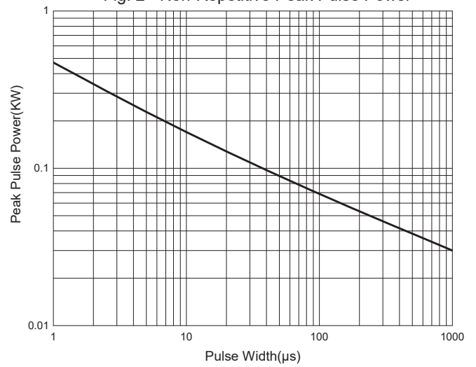
Fig. 2 - Non-Repetitive Peak Pulse Power
