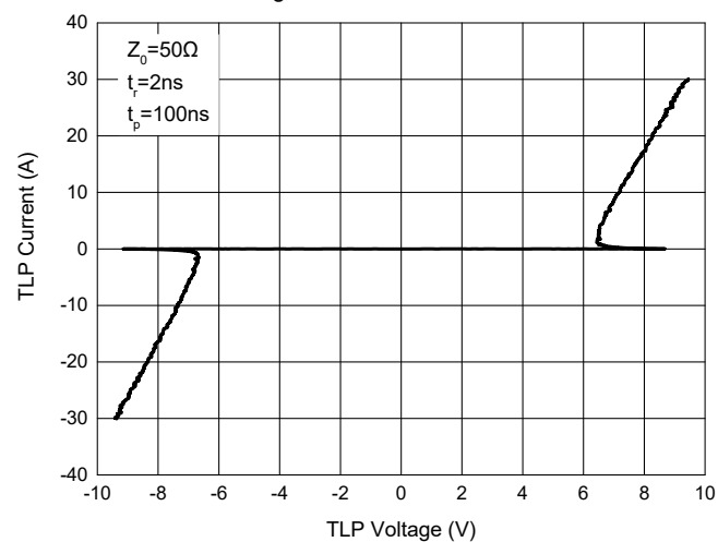
Fig. 4 - TLP Measurement
