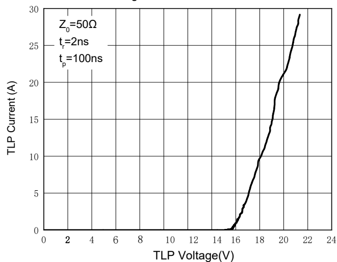
Fig. 5 - TLP Measurement
