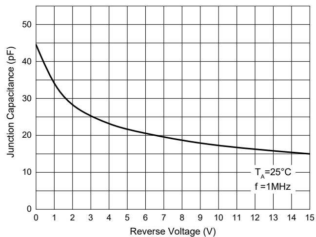
Fig. 3 - Capacitance Characteristics
