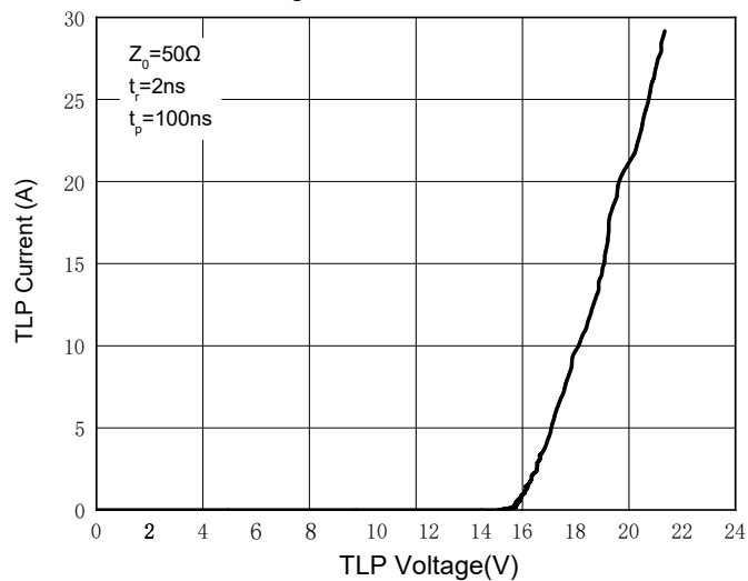
Fig. 5 - TLP Measurement
