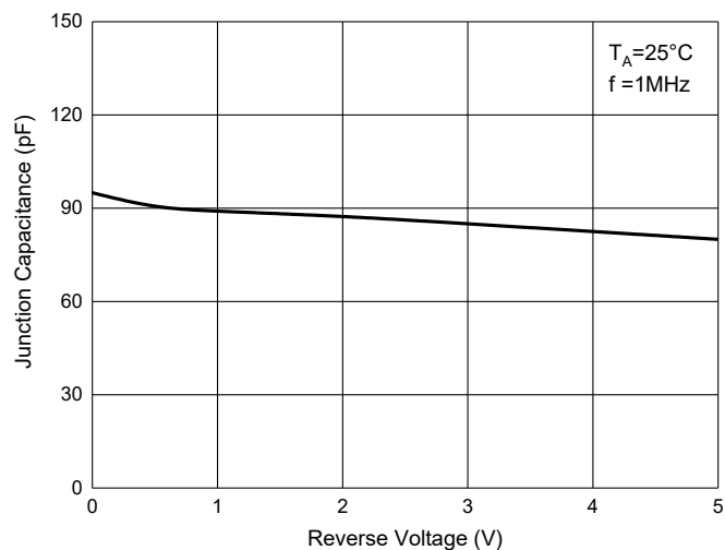
Fig. 4 - Capacitance Characteristics
