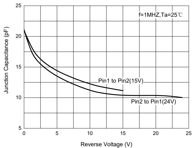
Fig. 4 - Capacitance Characteristics
