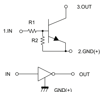
Internal Structure
