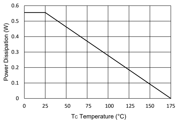
Fig.11 - PD Dissipation
