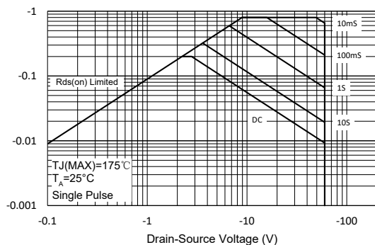
Fig.12 - Safe Operation Area
