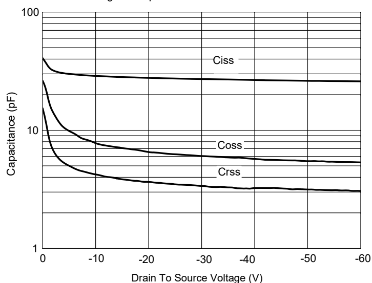
Fig. 5 - Capacitance Characteristics
