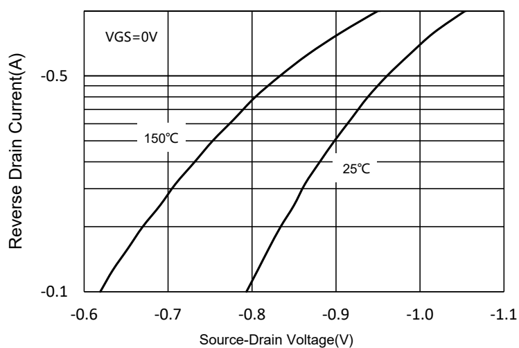
Fig.9 IS-VSD
