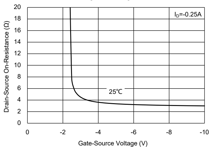
Fig.3 Rdson-Vgs
