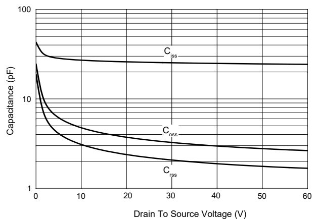
Fig.5 - Capacitance Characteristics
