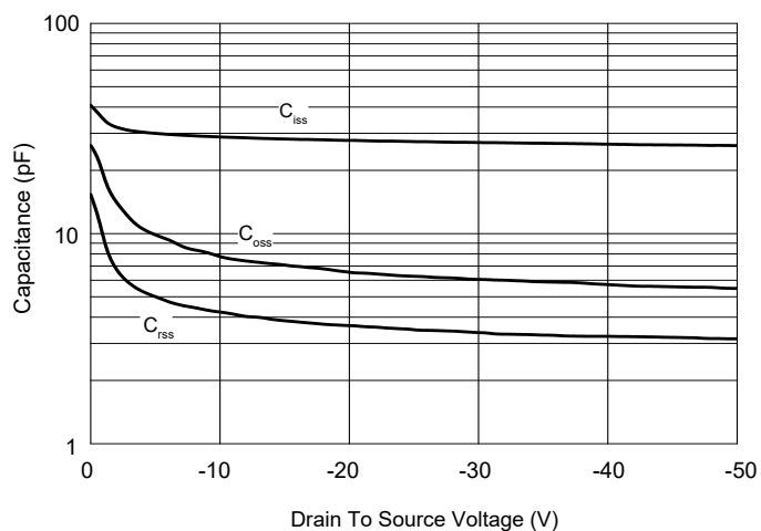
Fig. 5 - Capacitance Characteristics
