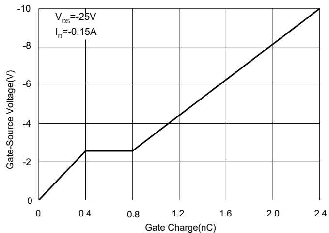
Fig.6 Gate Charge
