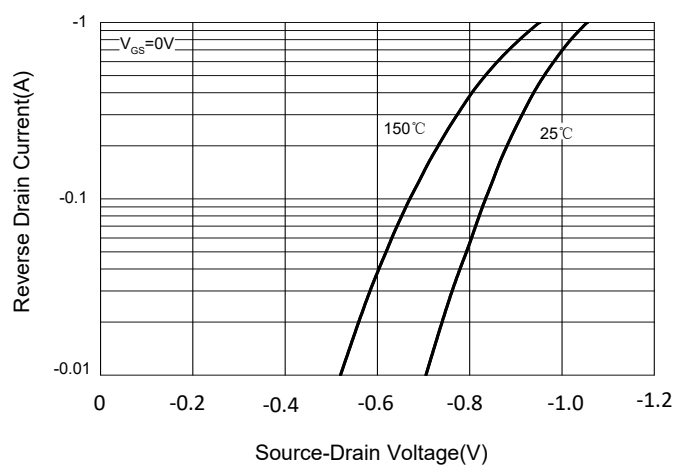
Fig.9 IS-VSD
