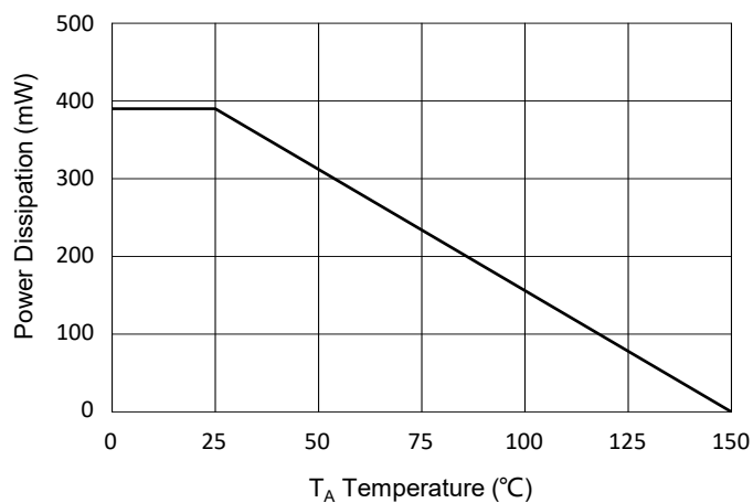
Fig.11 - PD Dissipation
