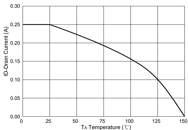
Fig. 10 - Drain Current
