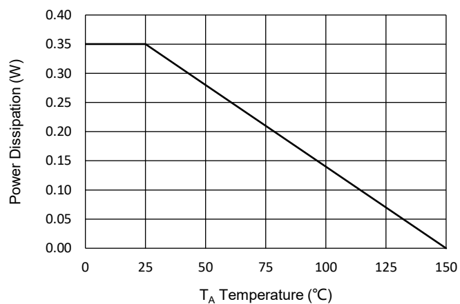
Fig.11 - PD Dissipation
