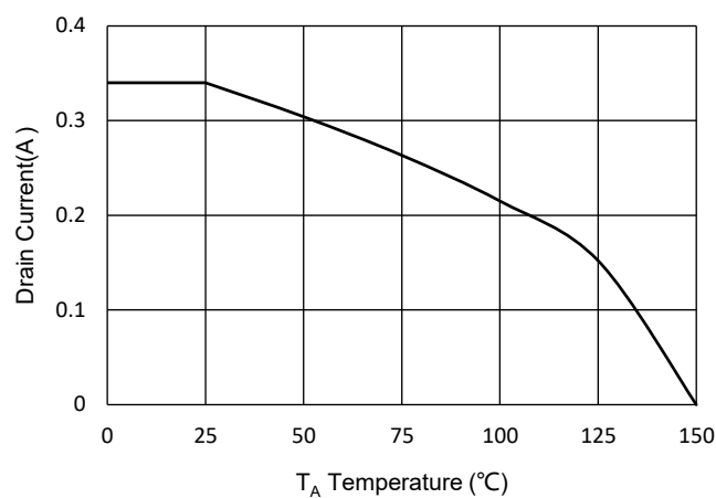
Fig.10 - Drain Current
